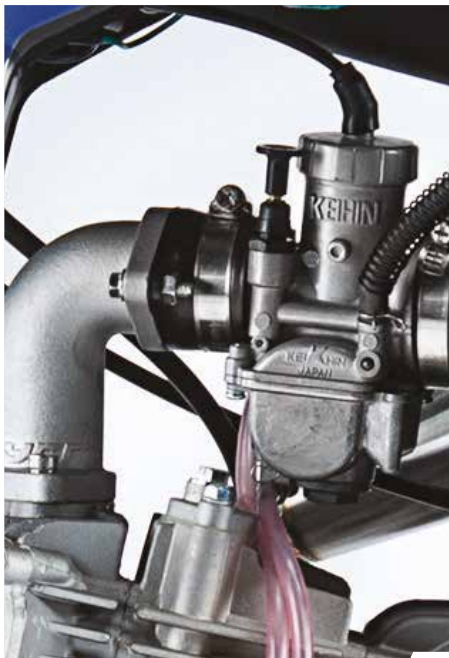
FUEL LINE RED/ ORANGE/ BLUE/ GREEN YELLOW/ PINK DURITE ESSENCE ROUGE/ ORANGE/ BLEUE VERTE/ JAUNE/ ROSE
